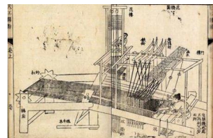
Fig. 4. The handloom Hwaru-Do(花樓圖) in Cheon-Gong-Gae-Mul(天工開物) of Ming Dynasty[15]
