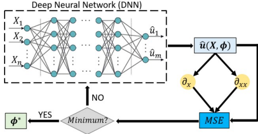
Fig. 1. Architecture of PINN. The neural networks can approximate the solution \hat{U} of differential equation. The idea behind PINN is to train the network using automatic differentiation.
