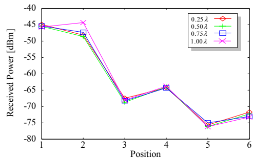
(a) Received Power
