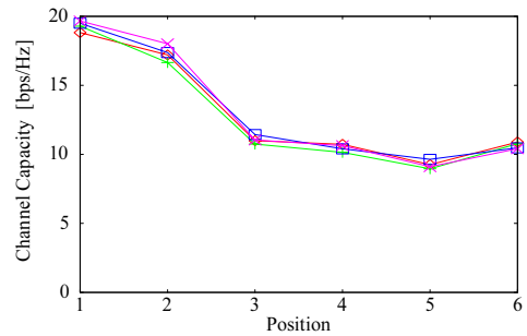
(b) Channel Capacity
