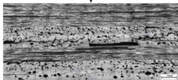
(b) Panel with kevlar/epoxy laminates
