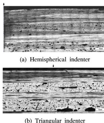
[Fig. 9] Impact damage in base panel at 60J
