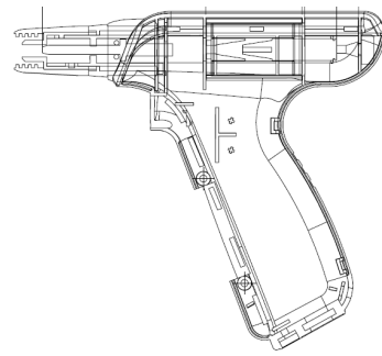
(a) 채혈기 평면도 (a) The drawing of a lancing device
