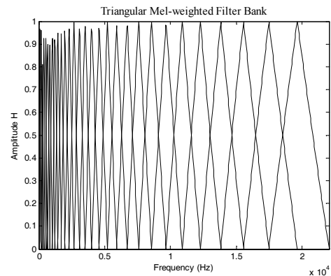
[그림 10] 정규화된 삼각 Mel-weighted Filter Bank [Fig. 10] The normalized Triangular Mel-weighted Filter Bank
