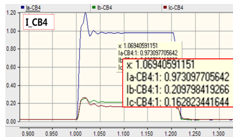
(a) 1선지락전류(I_CB4) (a) A single line ground faults current(I_CB4)
