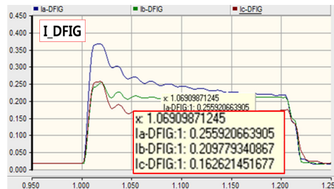
(b) 1선지락전류(I_DFIG) (b) A single line ground faults current(I_DFIG)
