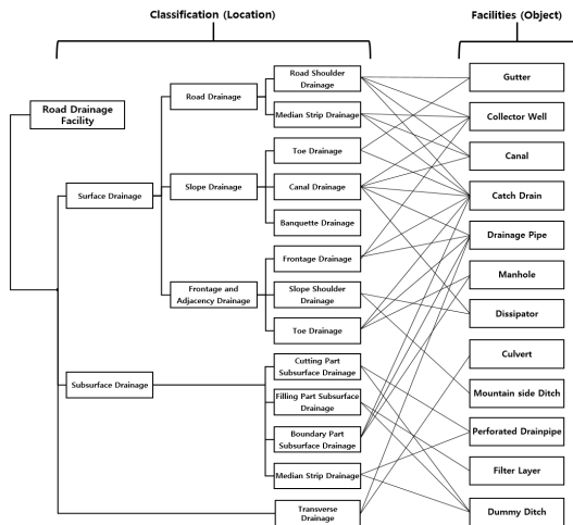
[Fig. 5] Classification of Drainage Facilities
