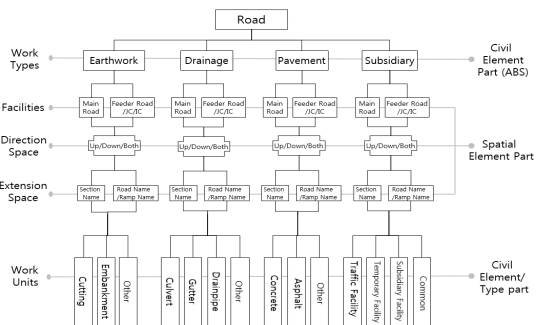
[Fig. 4] Work Breakdown Structure of Road Project
