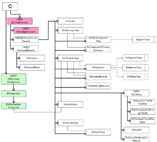
[Fig. 3] A Part of IFC-Shield Tunnel
