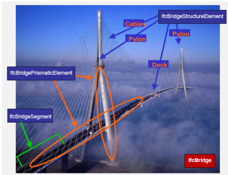
[Fig. 2] A Concept of Extension IFC Schema for Bridge
