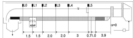
[Fig. 2] Experiment apparatus by Song
