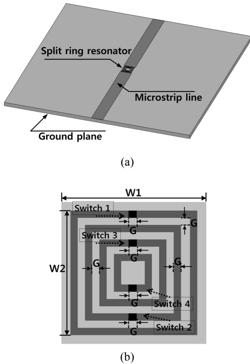
[Fig. 1] Proposed cross-polarized SRR filter structure. (a) microstripline with quad rings SRR (b) Reconfigurable SRR structures with four artificial switches
