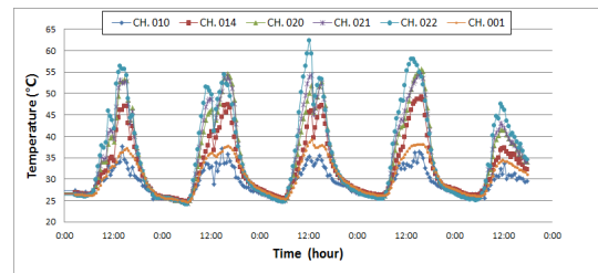
[Fig. 5] Temperature variation at the girder model
