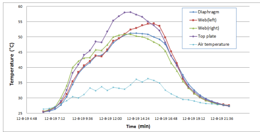
[Fig. 6] Temperature variation at measured points
