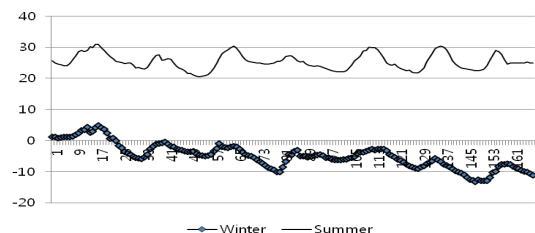
Fig. 3. Hourly Temperature: Winter, Summer (Winter: 2012. 12. 3(Mon) ~ 12. 9, Summer: 2013. 7. 1(Mon) ~ 7.7)
