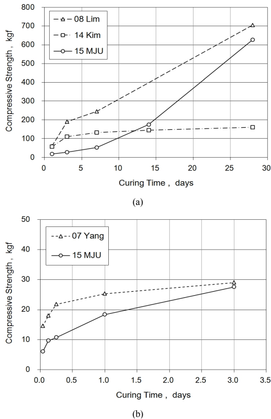
Fig. 5. Comparison of uniaxial compressive strength - LW (a)Long term (b)Short term
