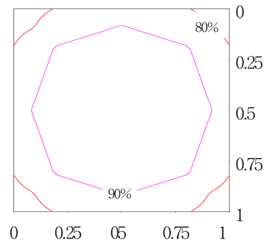
Fig. 8. Isometric lux
