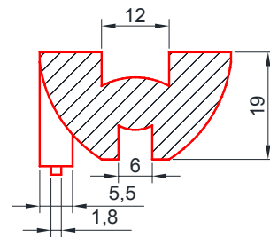
(b) Section
